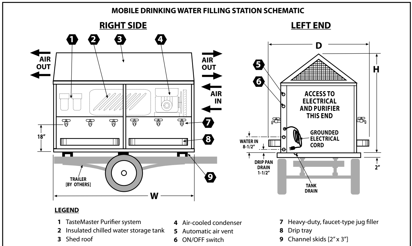
TYPICAL DRINKING WATER FILLING STATION
